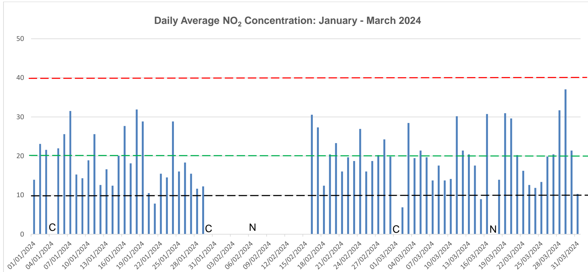
Figure 4 Daily Average NO 2 Q1 2024 On-Site Air Quality Station
