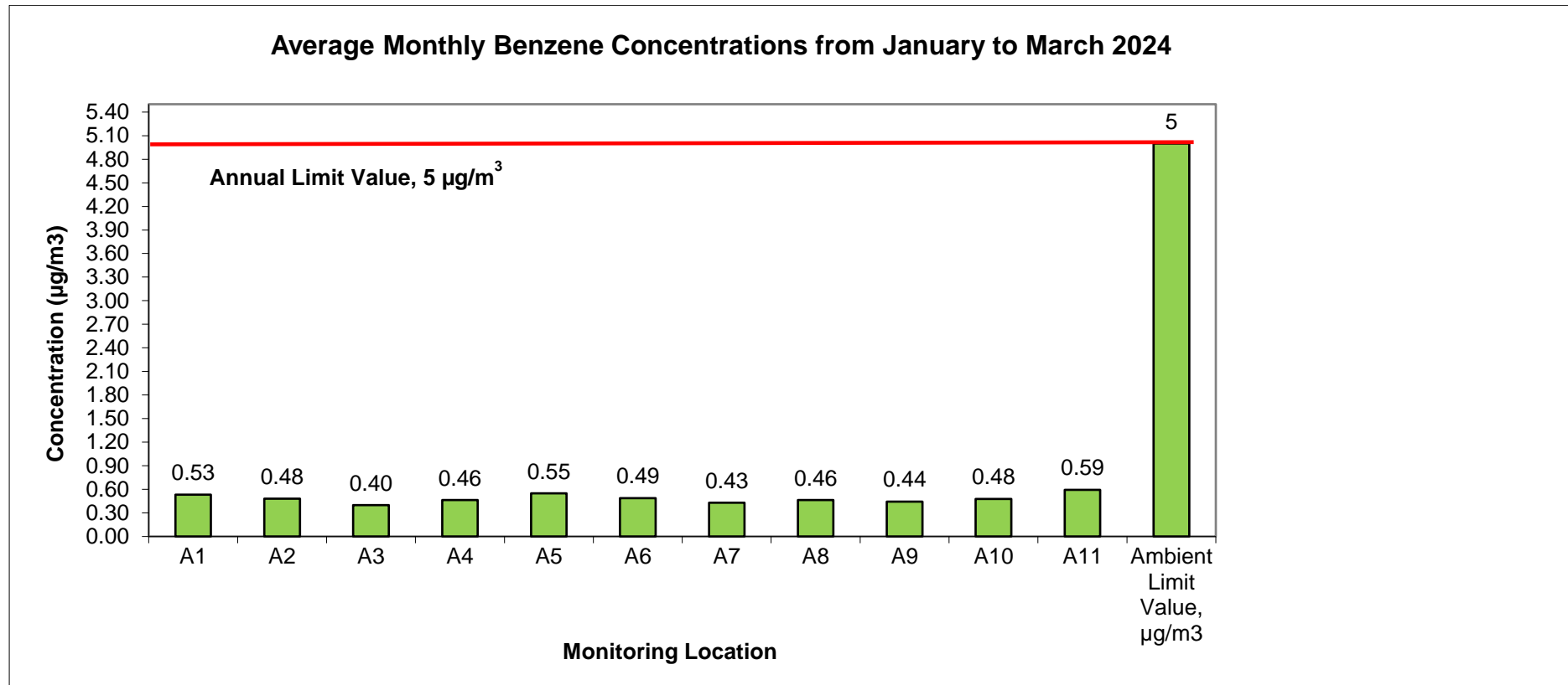
Figure 3 Average Monthly Benzene (C 6 H 6 ) Concentrations Q1 2024
