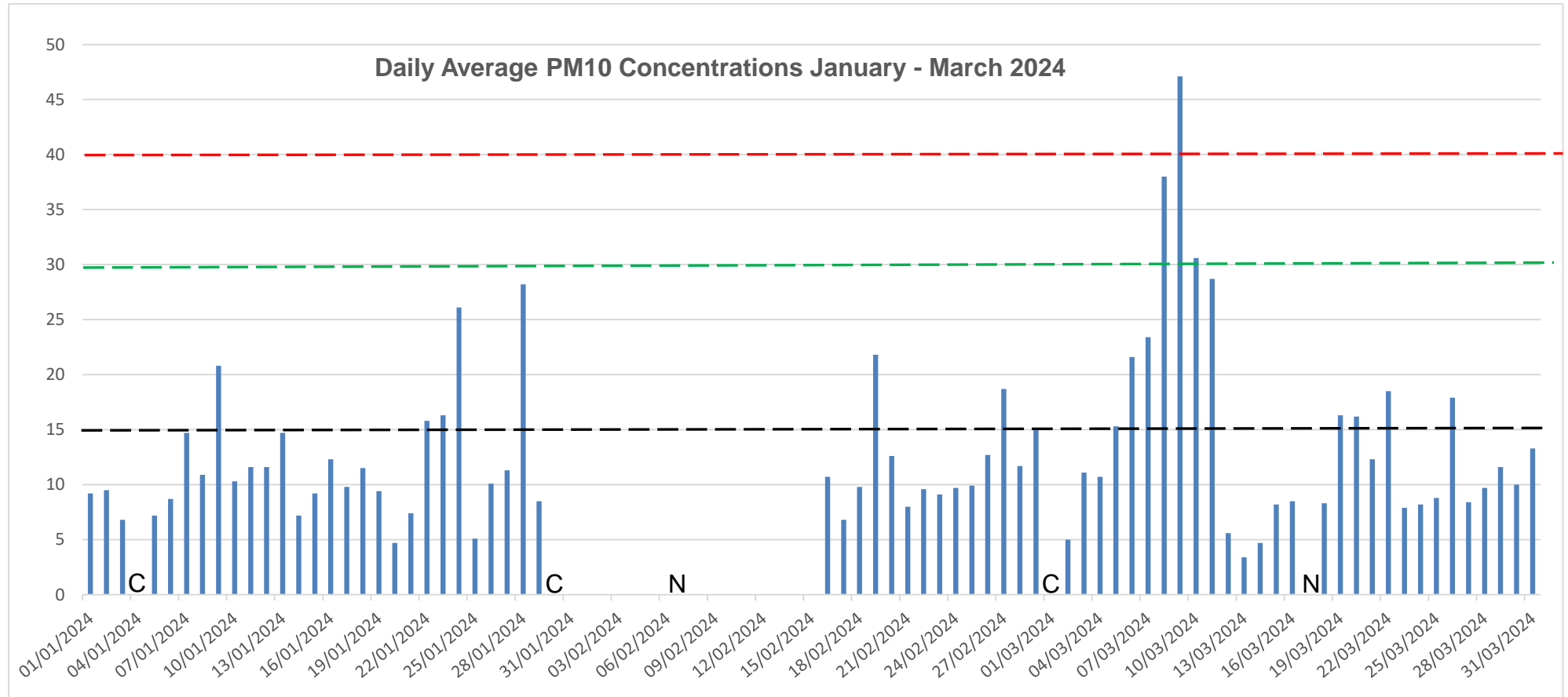
Figure 5 Daily Average PM 10 Q1 2024
