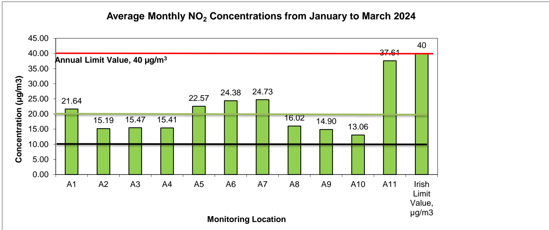
Figure 2 Average Monthly NO 2 Concentrations Q1 2024
